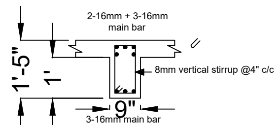
Beam at support section 3-3
