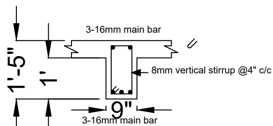
Beam at mid section 2-2
