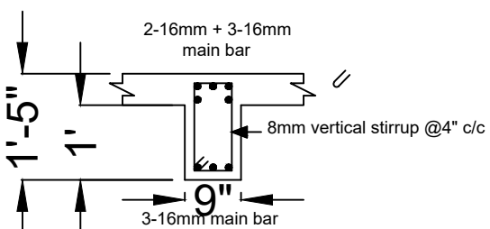
Beam at support section 1-1
